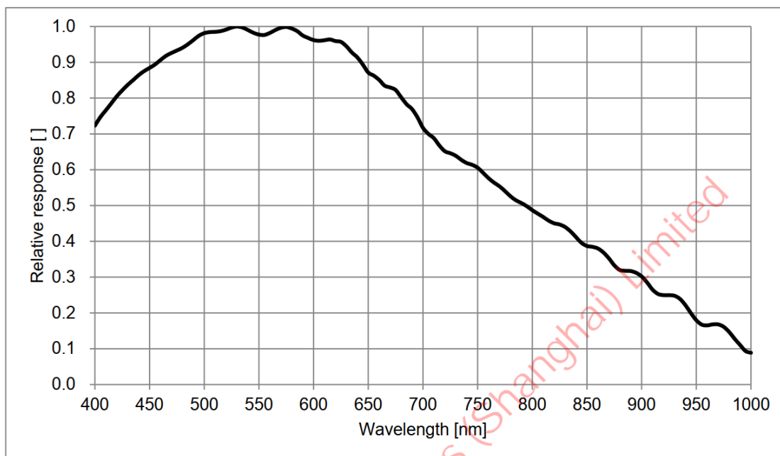
Relative QE Curve for ASI294MM
